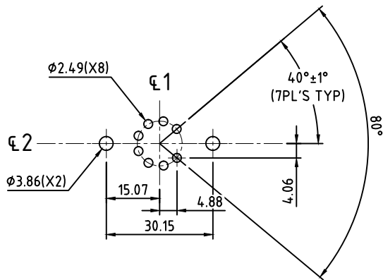
HOLE PATTERN
